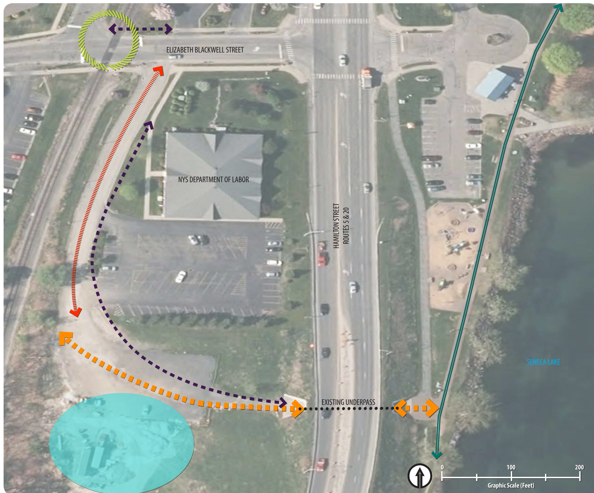
FIGURE 14B CITY-TO-LAKE CONNECTIVITY EXISTING UNDERPASS: CONCEPT PLAN
